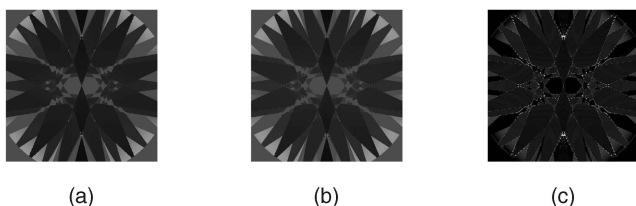
Fig. 5. Number of steps taken along each ray for a Barth 10th-order surface for the AMP algorithm (a) without silhouette adaptation, (b) with it, and (c) difference image scaled by 2 for legibility. Darker color indicates fewer steps.
